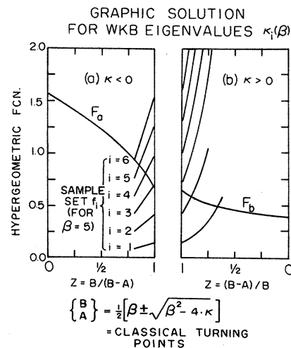
FIG. 14. Graphical solution for WKB eigenvalues \kappa_i^{\text{WKB}} .
