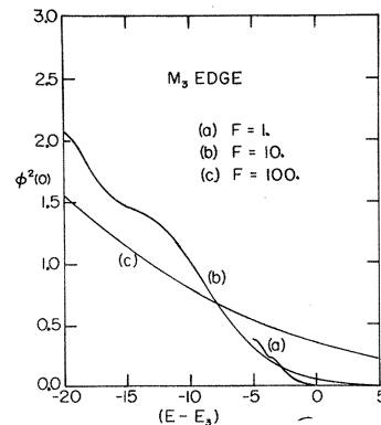
FIG. 13. Field dependence of optical absorption near an M_3 -type edge for F = \mathcal{E}/\mathcal{E}_T = 1.0, 10.0, and 100.0 . By comparison of the M_0 and M_3 edges, it is evident that the electron-hole interaction enhances the electric-field-induced oscillations near an M_0 edge (positive effective masses) and quenches these oscillations near an M_3 edge (negative effective masses).
